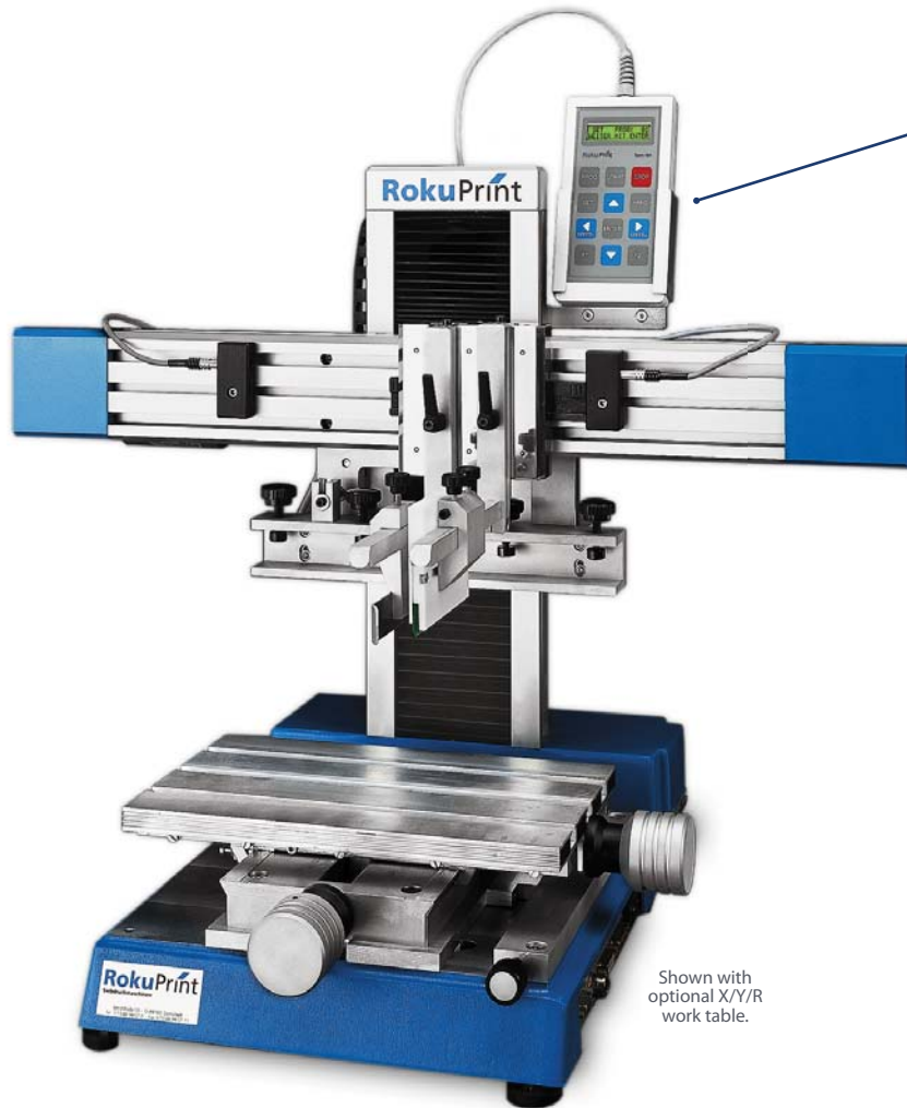
User-friendly handheld controller makes programming and set-up a simple task
